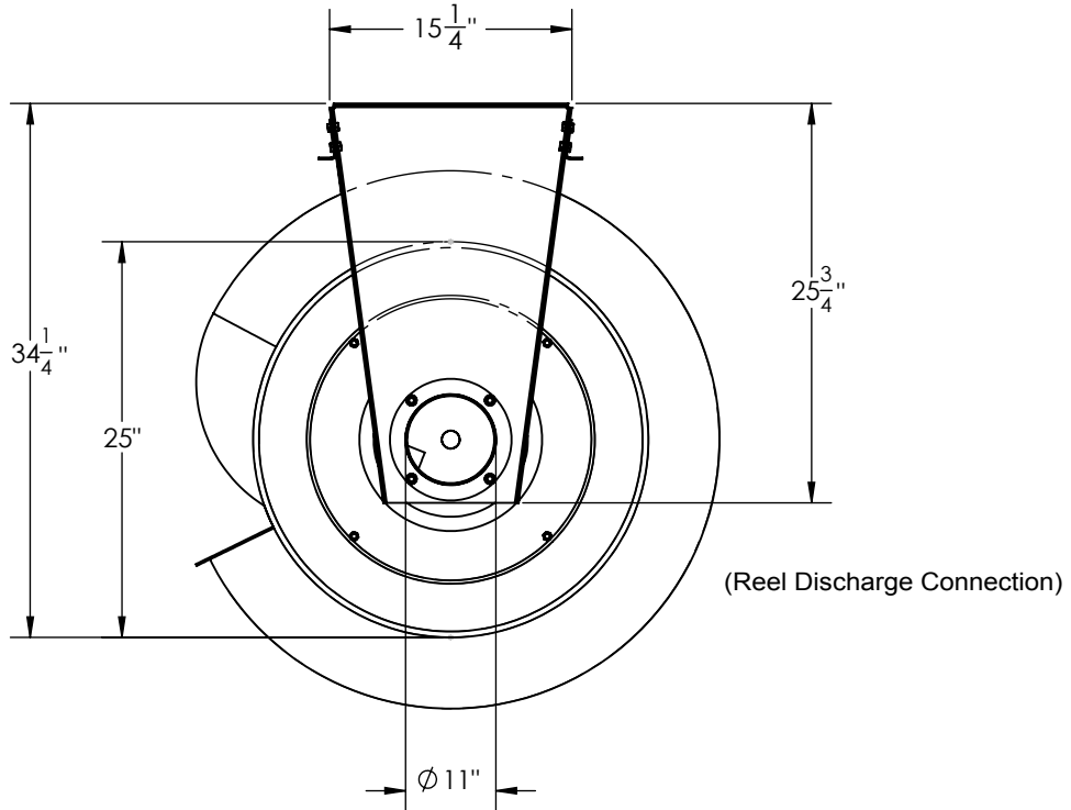
SIDE/END VIEW
