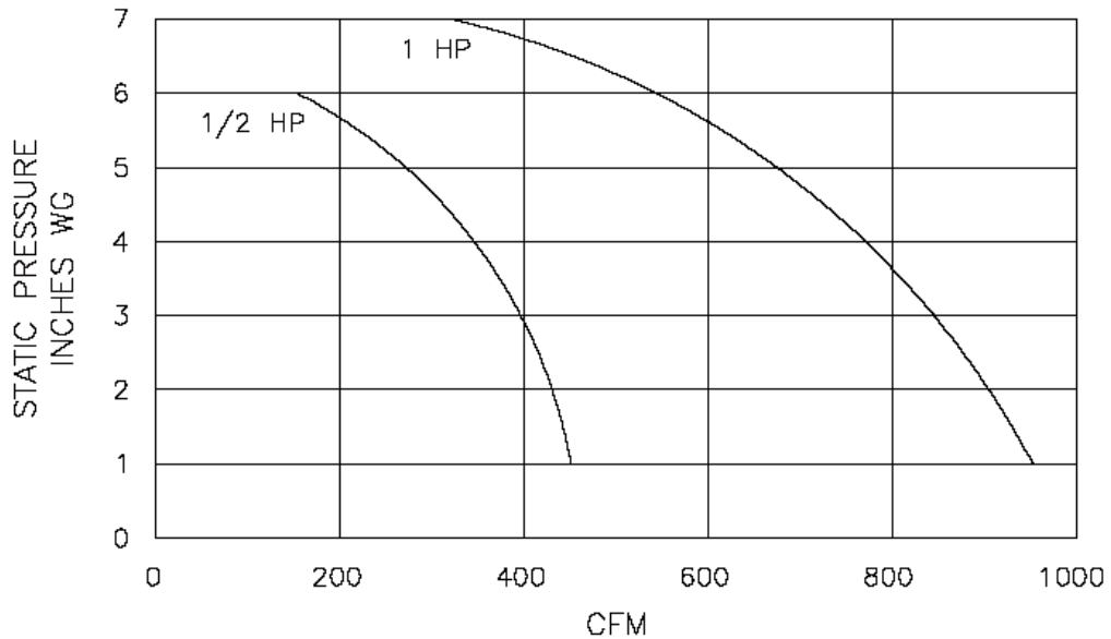
FAN SERIES DMHR PERFORMANCE GRAPH FOR 1/2 HP & 1 HP PRESSURE BLOWERS
