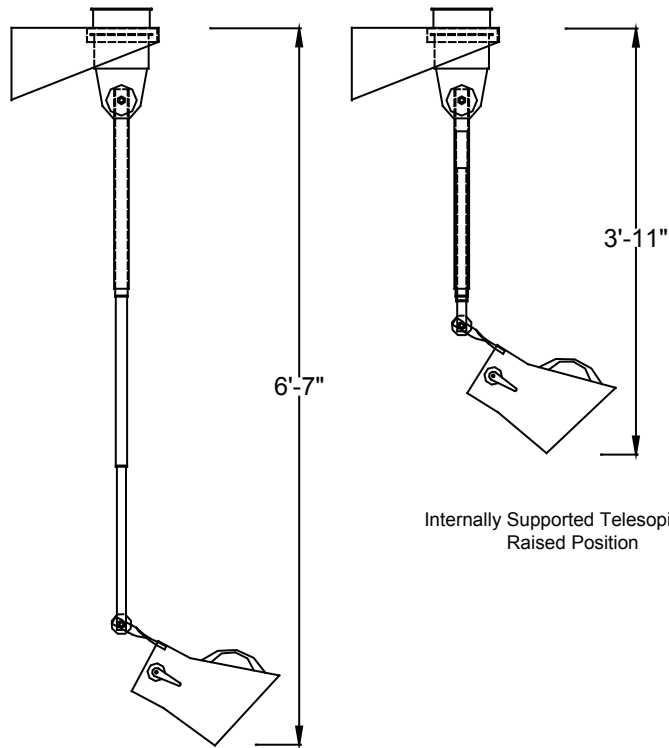
Internally Supported Telescopic Arm Extended Position
