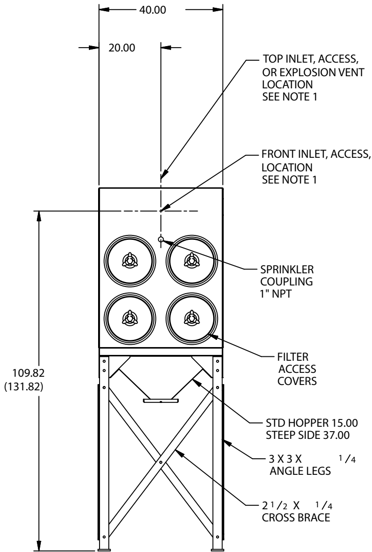
FRONT VIEW
