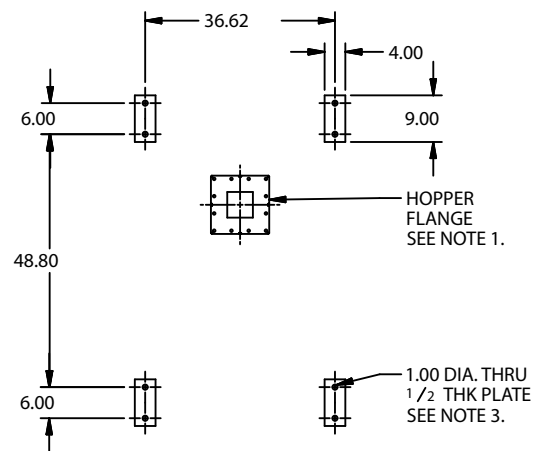
ANCHOR BOLT PLAN
