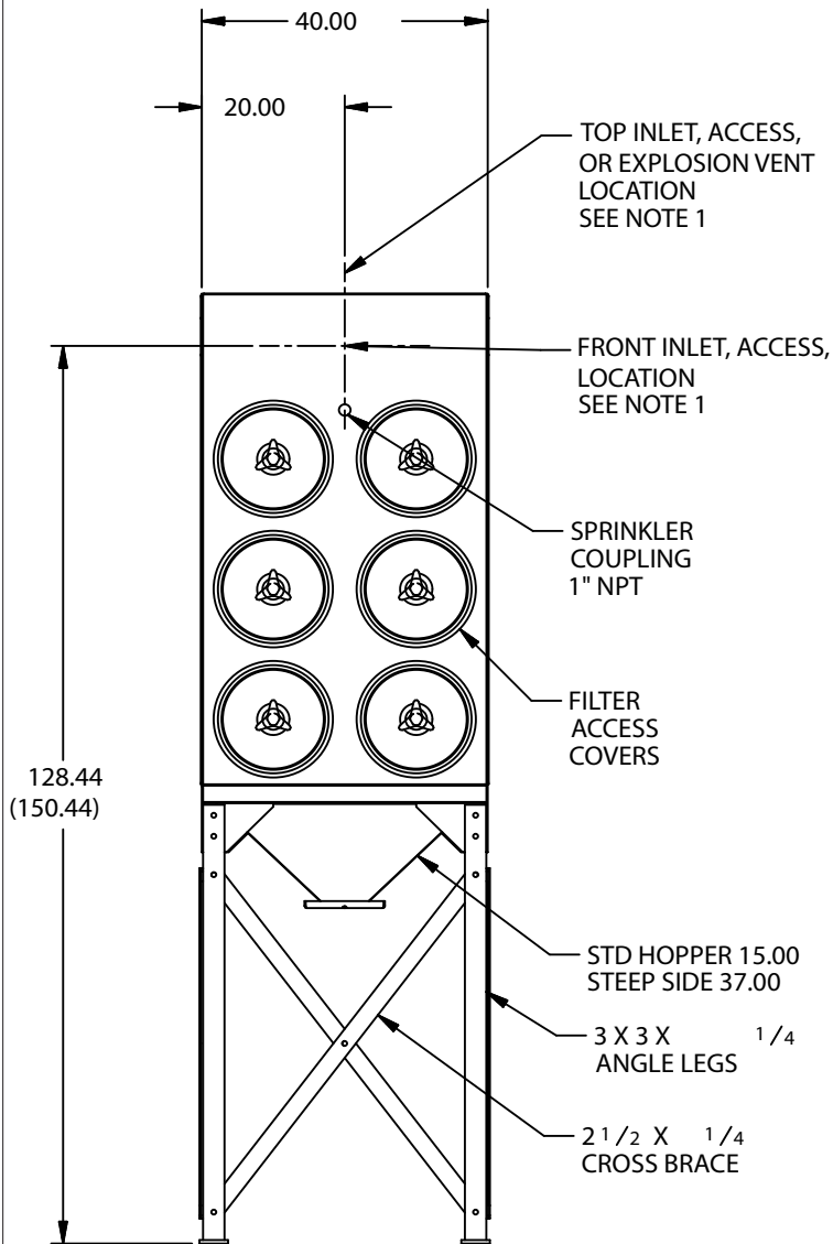
FRONT VIEW
