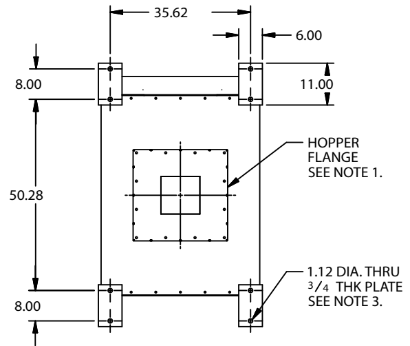
ANCHOR BOLT PLAN
