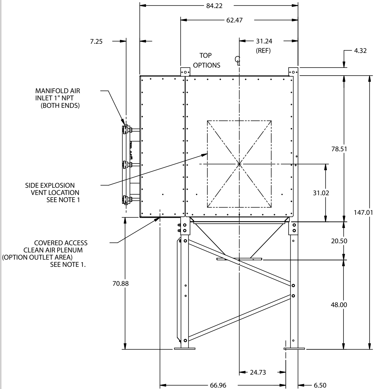
SIDE VIEW
