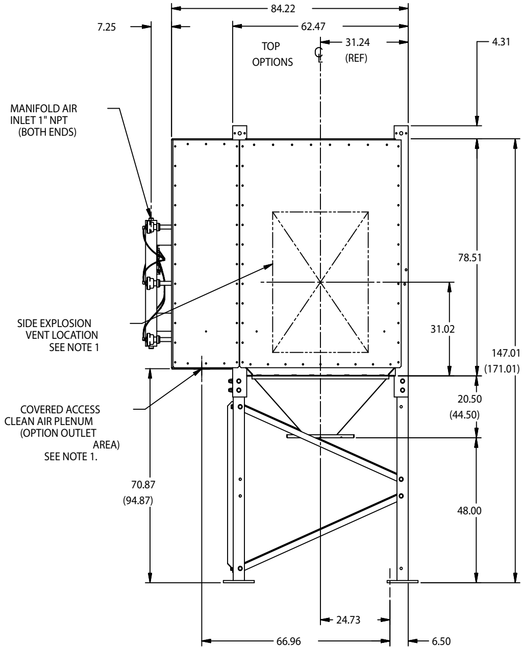
SIDE VIEW
